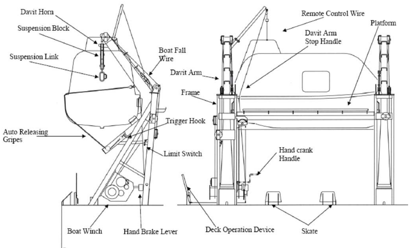
Fig. 1.1 Lifeboat davit arrangement
